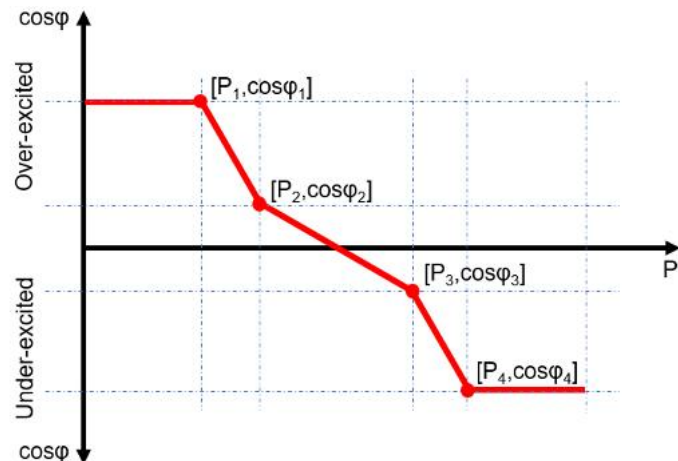
Abb. 193. Cos-phi(P)-Kurve
