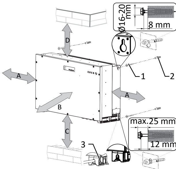
Abb. 19: Wandmontage
