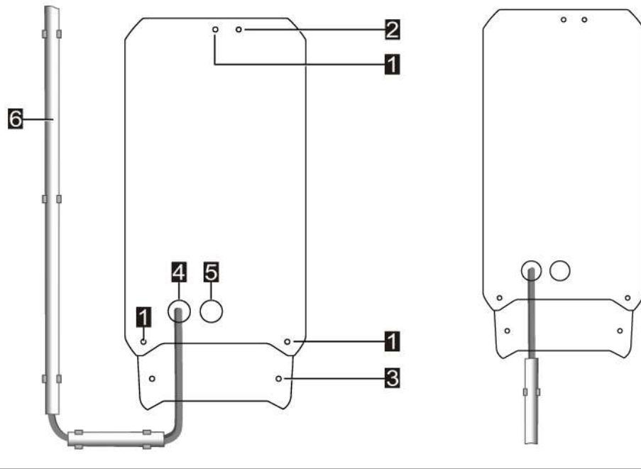
Fig. 8-3: Example: Mounting points and surface-mounted cable routing
