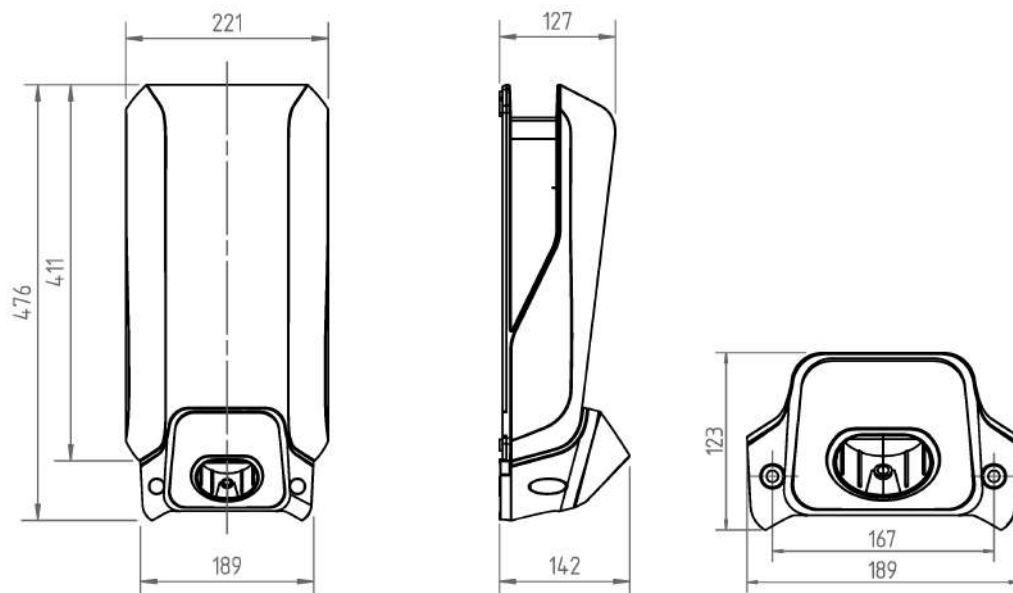
Dimensions in millimeter
