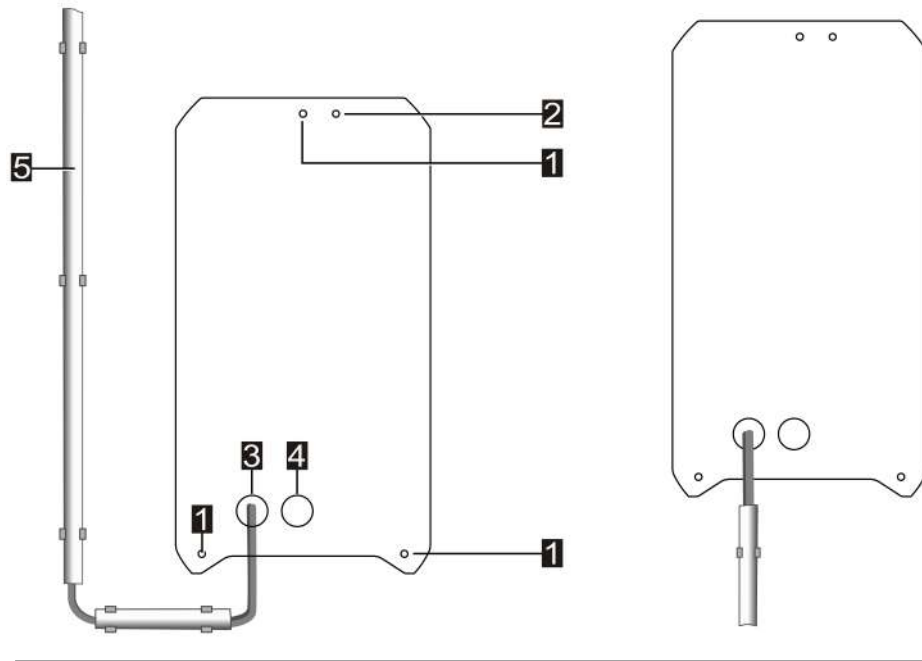
Fig. 8-4: Example: Mounting points and surface-mounted cable routing
