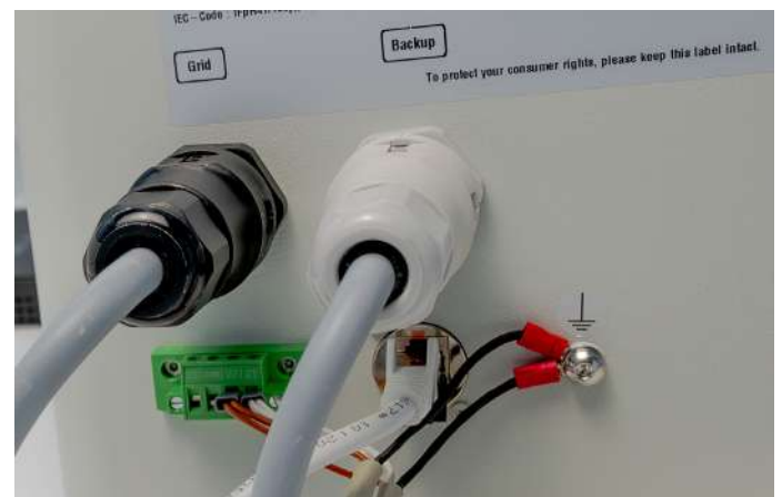
Fig. 56 Wired storage unit
