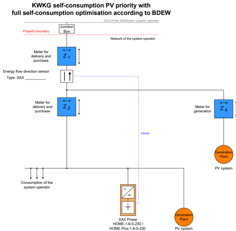
Fig. 30 Metering concept (two generation systems)
