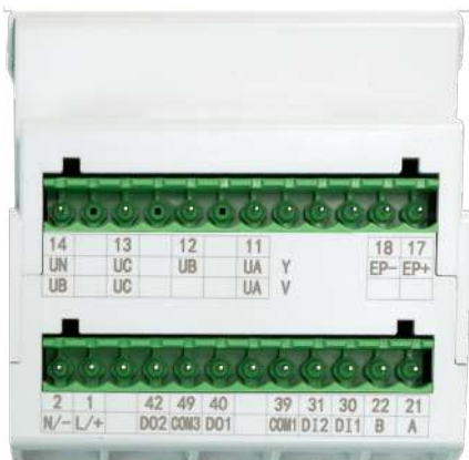
Fig. 41 ADW200: Top view
