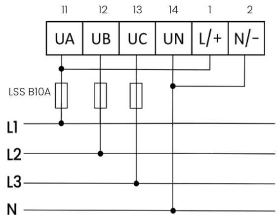
Fig. 44 Connection diagram for voltage measurement and power supply
