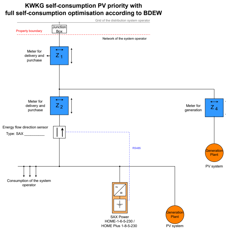
Fig. 31 Metering concept (two generation systems)
