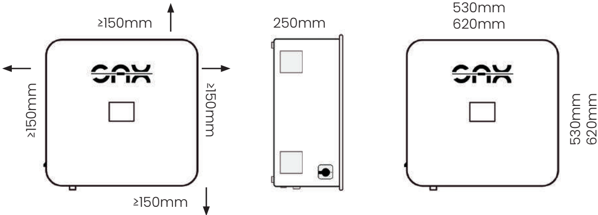
Fig. 13.3 Distance specifications and storage dimensions
