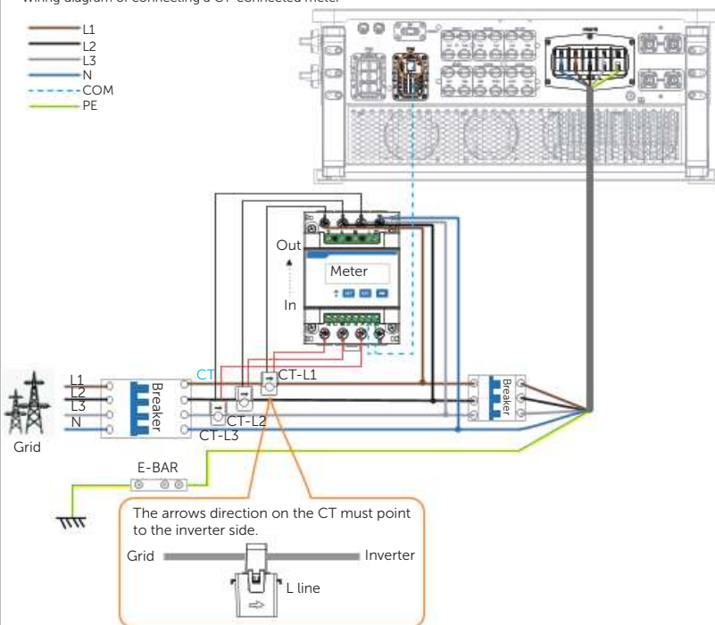
Wiring diagram of connecting a CT-connected meter
