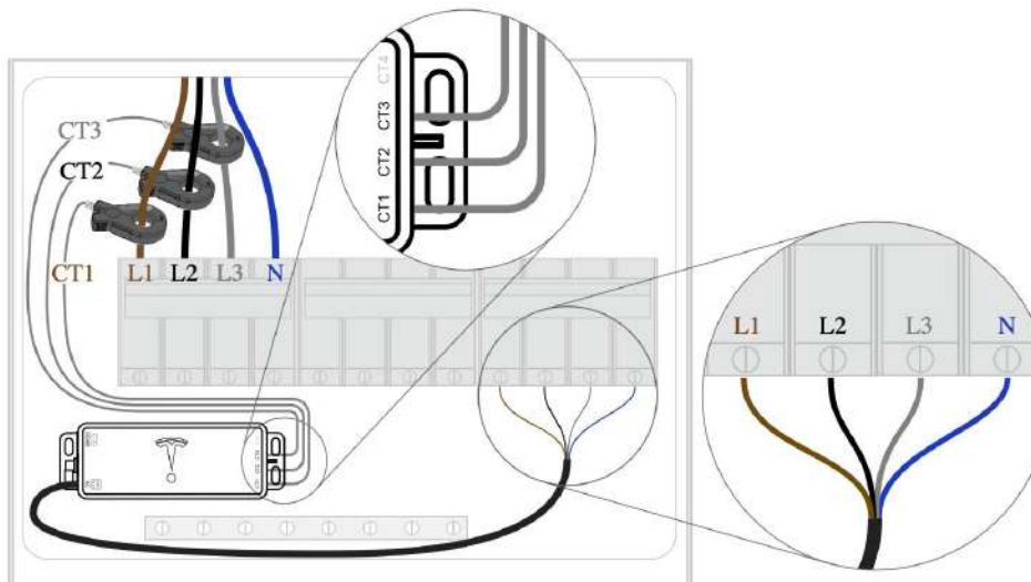
Figure 2. Configuration of remote meter inside panel - Three-phase
