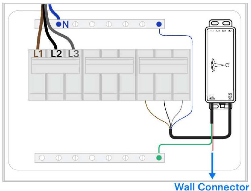
Figure 7. RS-485 Protective Earth Conductor Connected to Distribution Board Equipment Ground Board (Three Phase)
