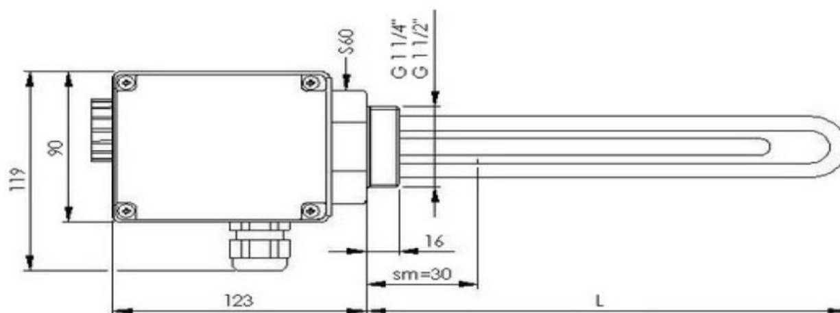
Figure 1. Dimensions — Heating element — 6 kW
