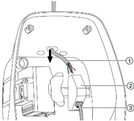
Fig. 15: Connecting the data line (example)
