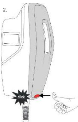
Fig. 22: Attach front cover - 2
