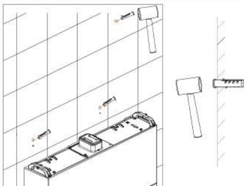
14 Knock expansion tubes into the wall with a rubber hammer.
