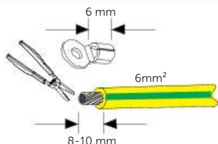
1 Strip the PE cable by wire stripper.
