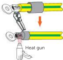
3 Crimp OT terminal and heat the heat-shrink tubing.
